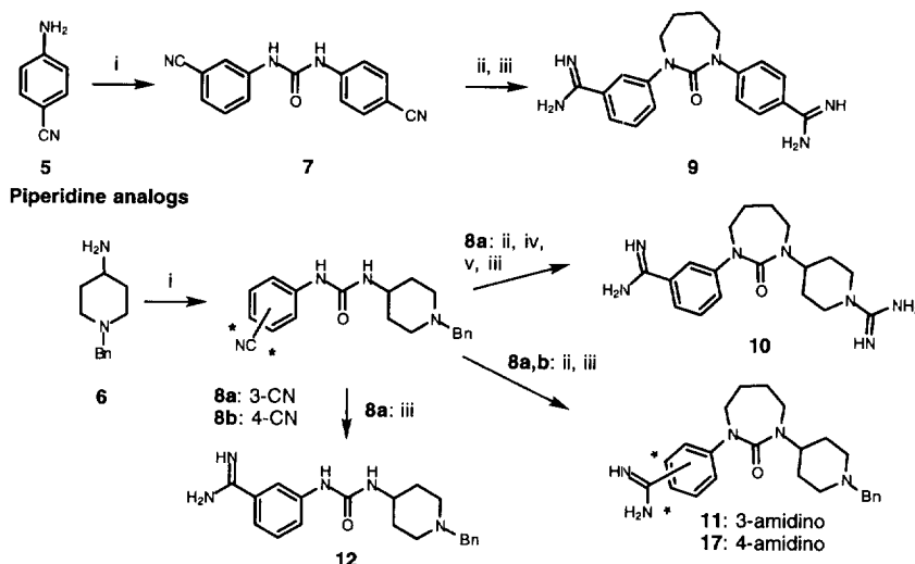
Scheme 1. Synthesis of 2,4-diazepin-3-one and acyclic target compounds.
